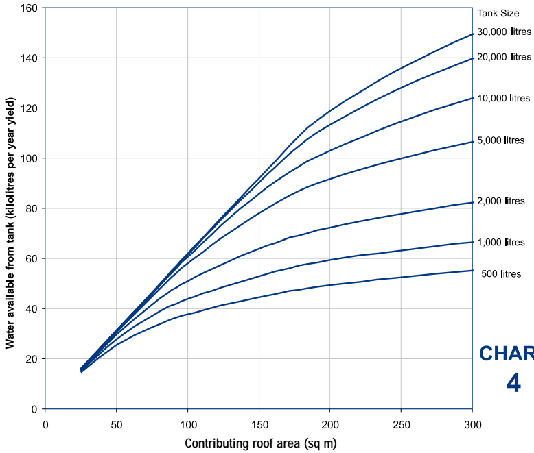
Tank usage: garden watering and toilet flushing
