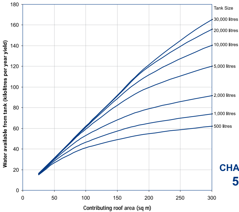
Tank usage: garden watering, toilet flushing and laundering
